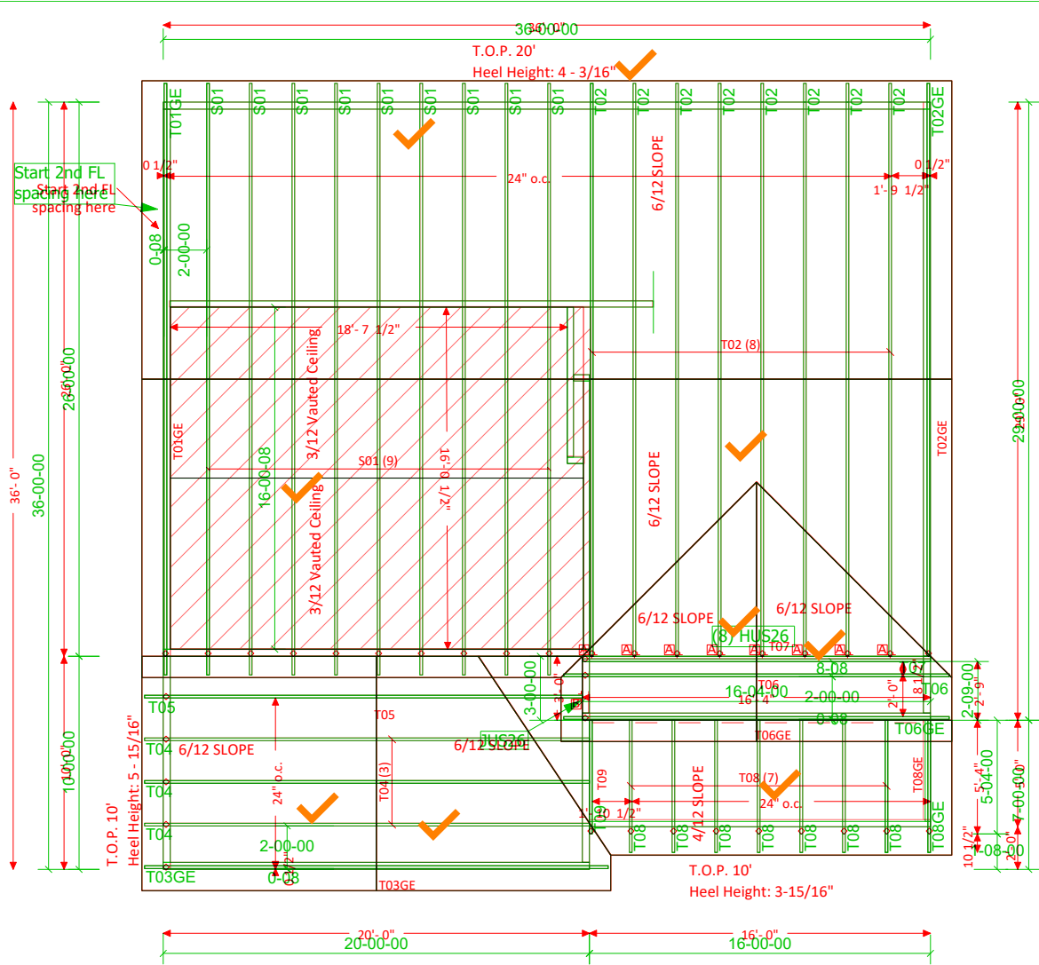
Truss Placement Plan
