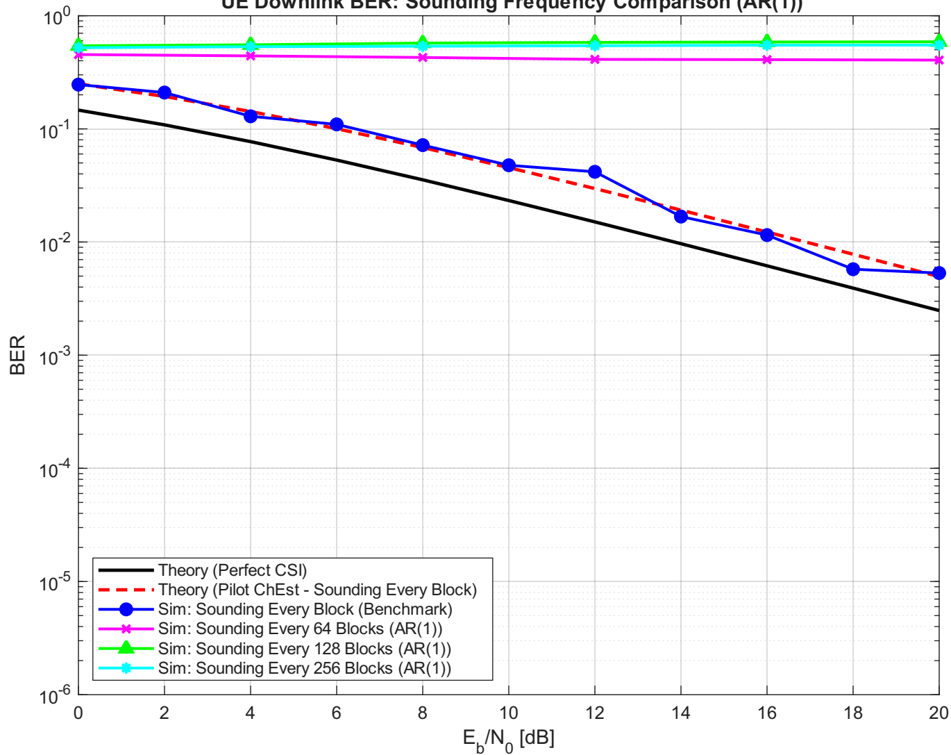
UE Downlink BER: Sounding Frequency Comparison (AR(1))
