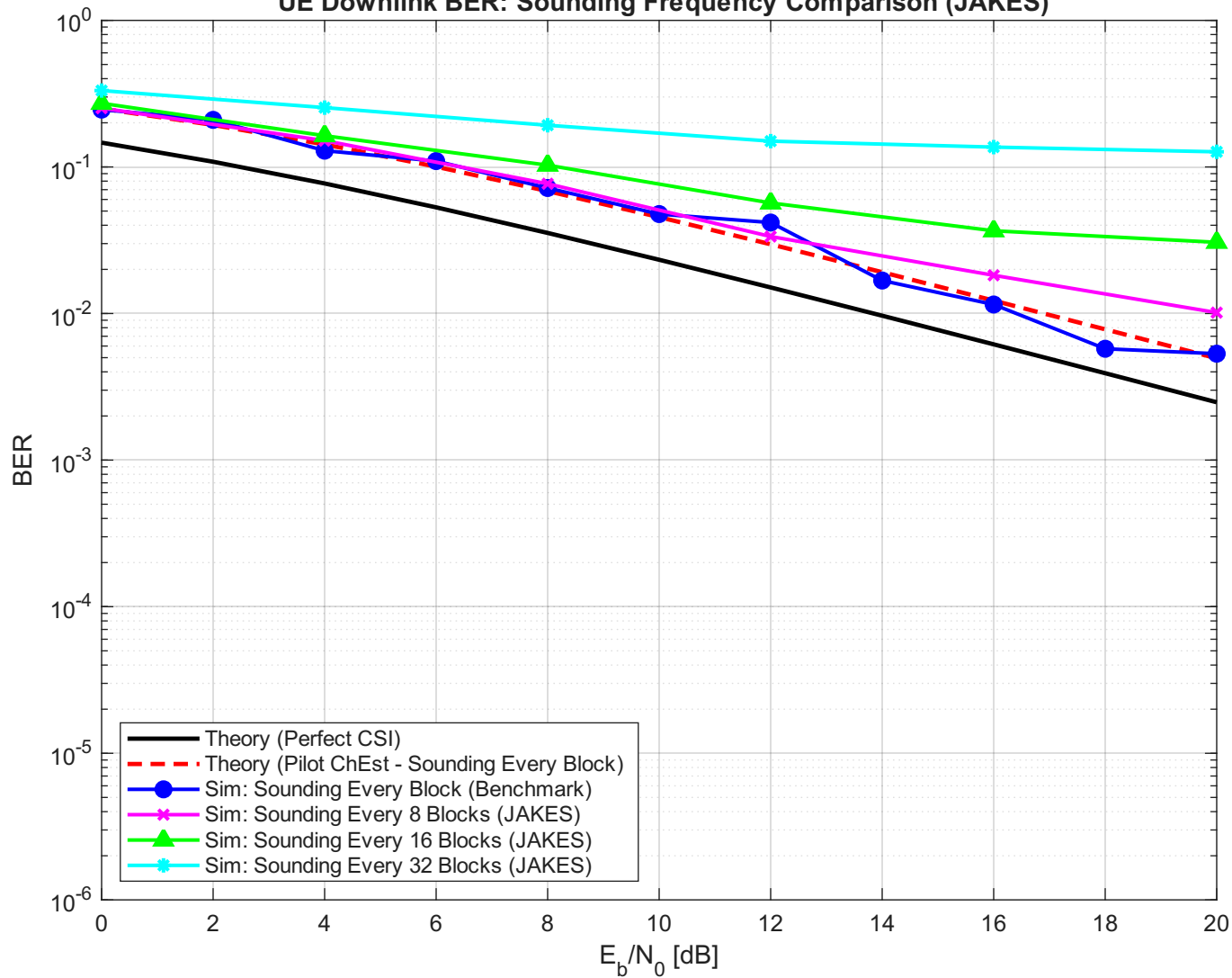
UE Downlink BER: Sounding Frequency Comparison (JAKES)
