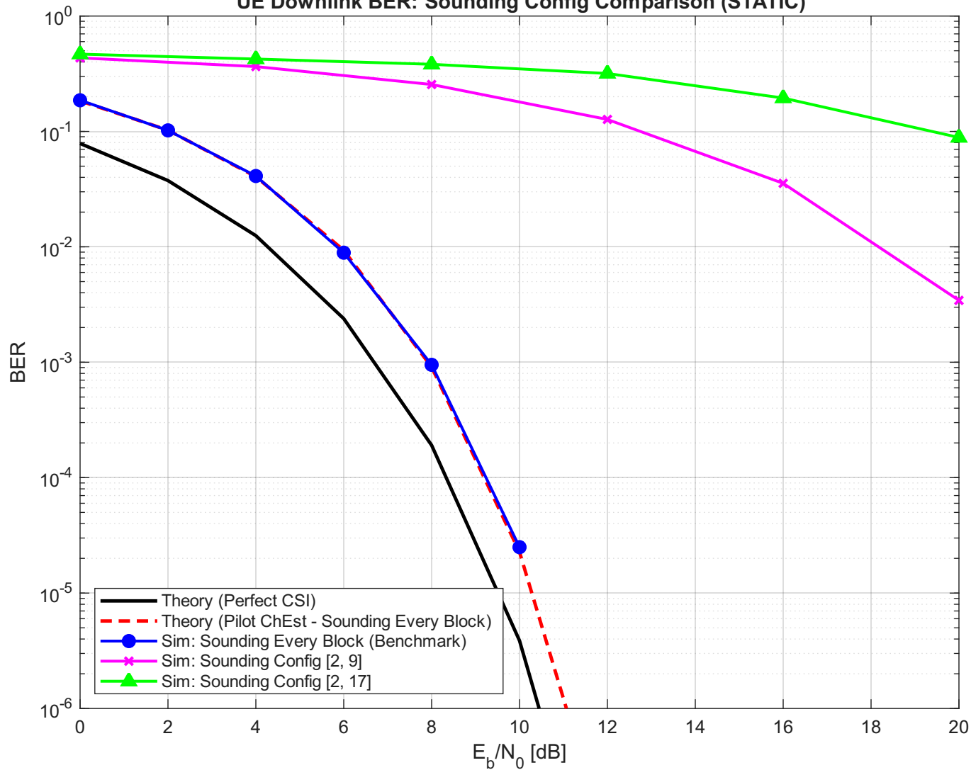
UE Downlink BER: Sounding Config Comparison (STATIC)
