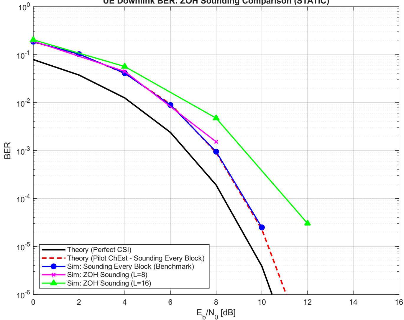
UE Downlink BER: ZOH Sounding Comparison (STATIC)
