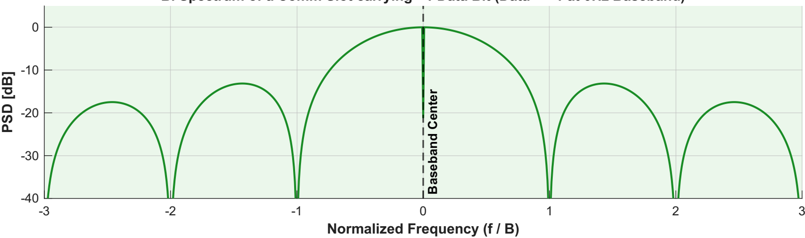
B. Spectrum of a Comm Slot carrying +1 Data Bit (Data = +1 at 0Hz Baseband)
