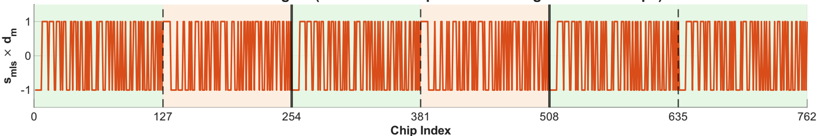
4. Baseband Waveform
