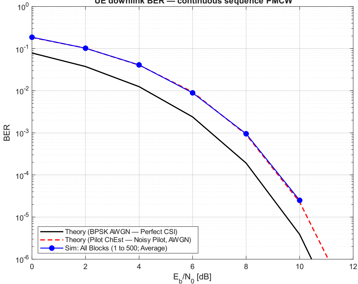
UE downlink BER — continuous sequence PMCW
