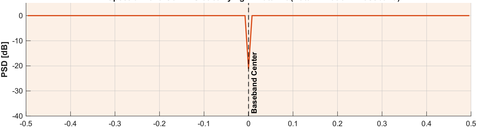
A. Spectrum of a Comm Slot carrying -1 Data Bit (Data = -1 at 0Hz Baseband)
