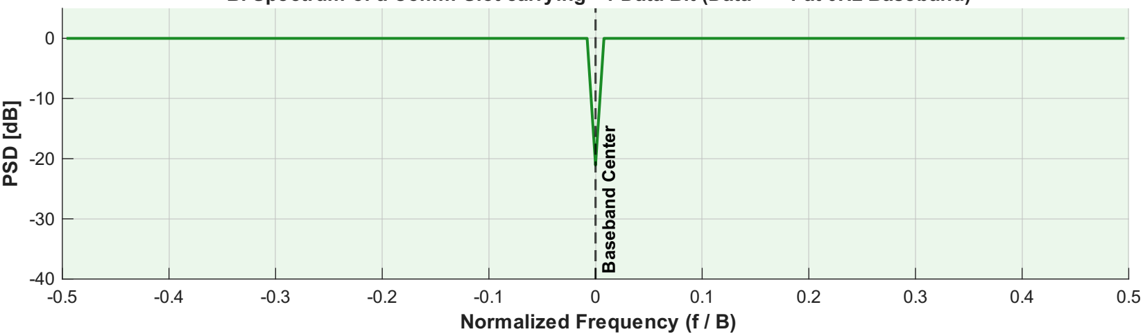
B. Spectrum of a Comm Slot carrying +1 Data Bit (Data = +1 at 0Hz Baseband)
