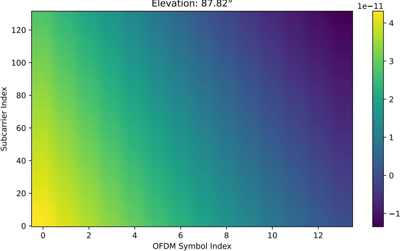
Precompensated Doppler: Real Part of Channel 0 (DUR) Elevation: 87.82°
