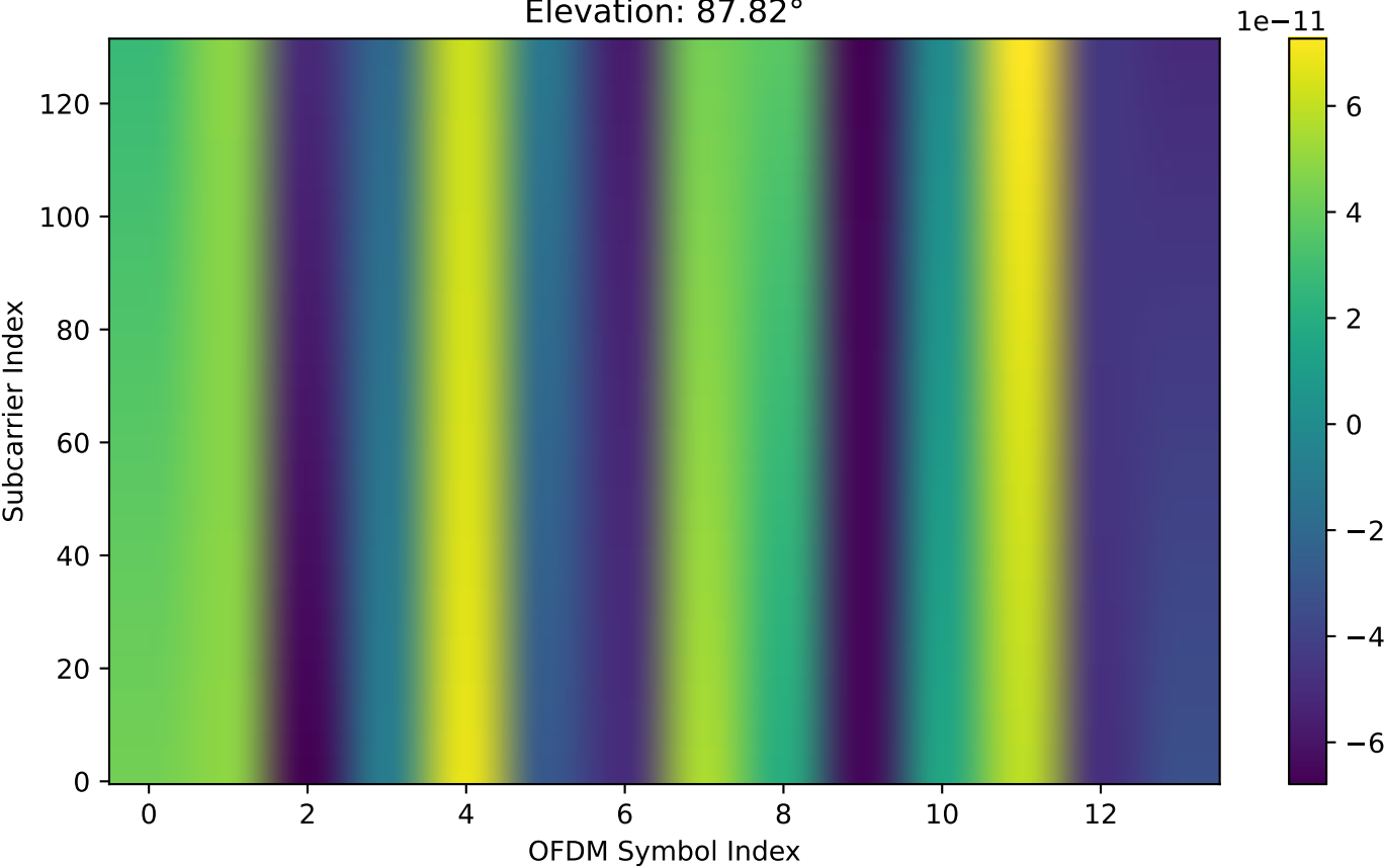
Full Doppler: Real Part of Channel 0 (DUR) Elevation: 87.82°
