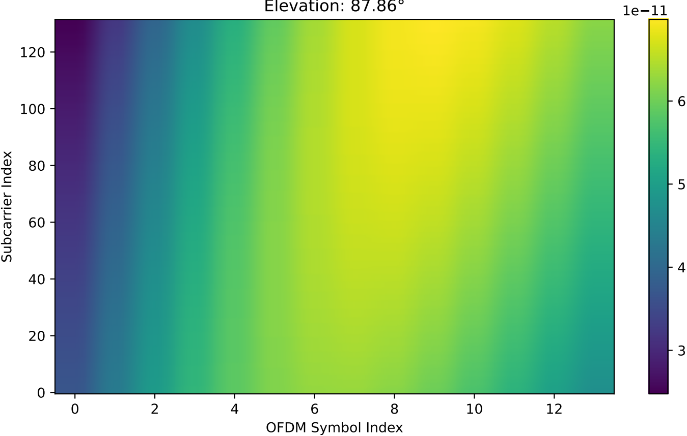
Precompensated Doppler: Real Part of Slot 0 Channel (DUR) Elevation: 87.86°
