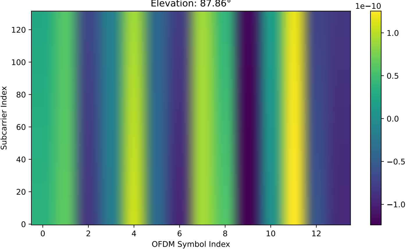
Full Doppler: Real Part of Slot 0 Channel (DUR) Elevation: 87.86°
