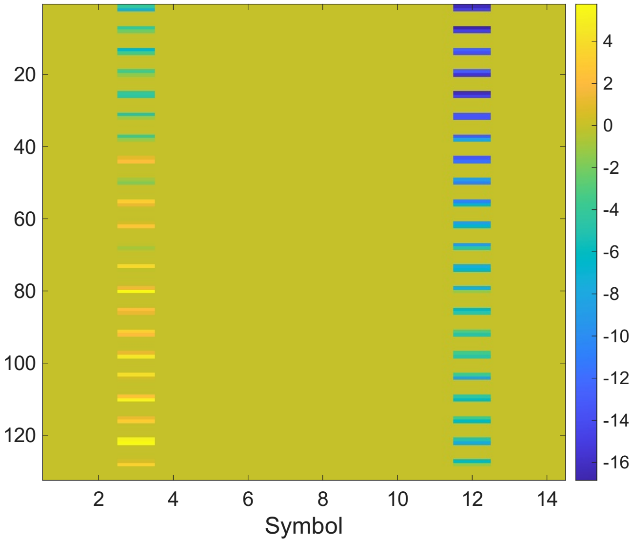
Sparse LS Estimated Channel H_{ls} (Sample 1)
