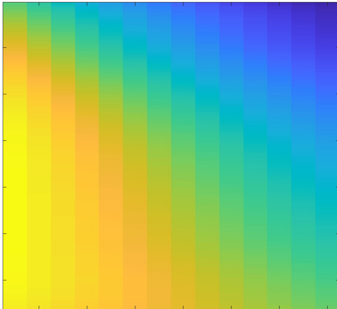
Effective Compensated Channel (Real Part) - Sample 1
