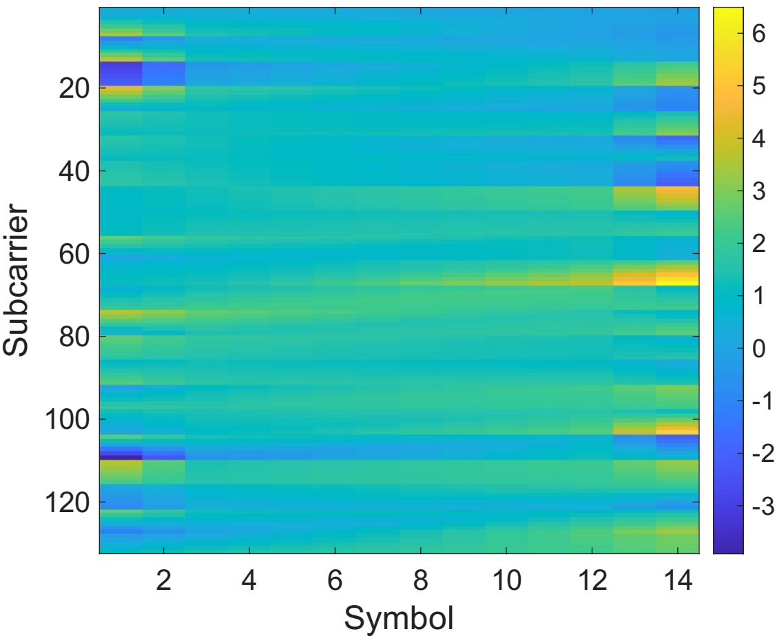
Linear Interpolation Estimated Channel H_{li} (Sample 1) \times 10^{-8}
