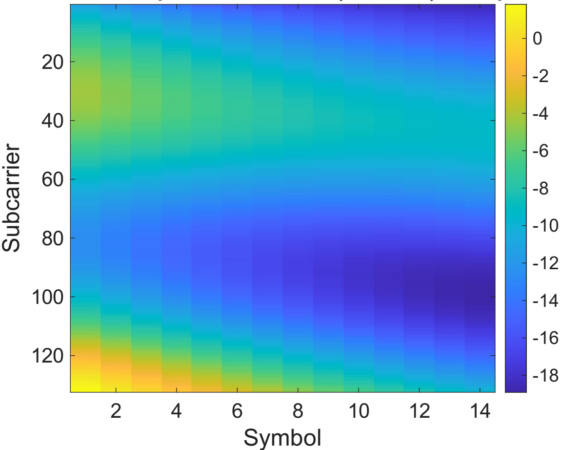
Effective Compensated Channel (Real Part) - Sample \times 10^{-9}
