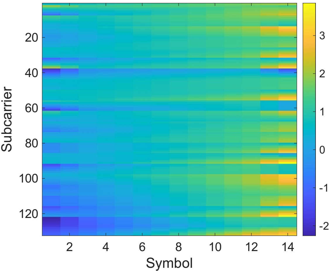
Linear Interpolation Estimated Channel H_i (Sample 1) \times 10^{-8}
