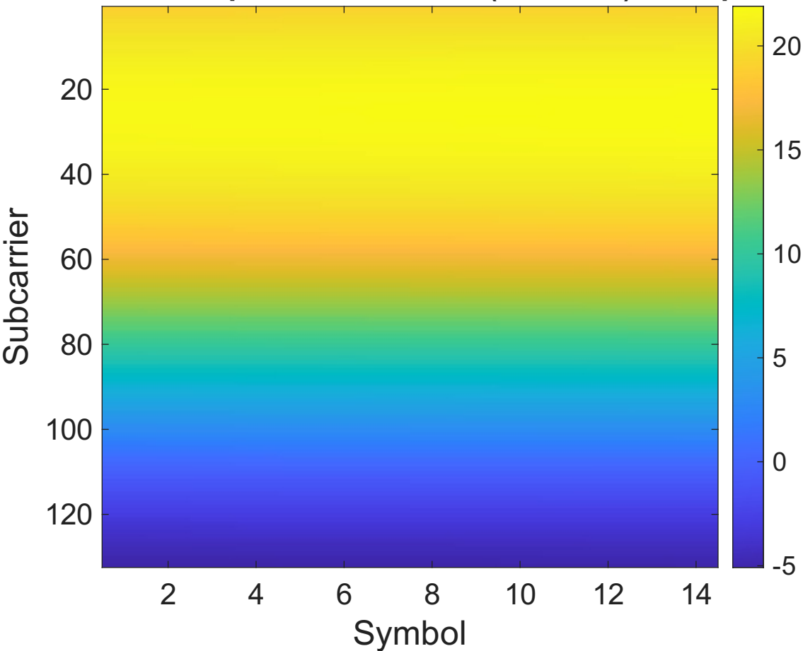
Effective Compensated Channel (Real Part) - Sample \times 10^{-9}
