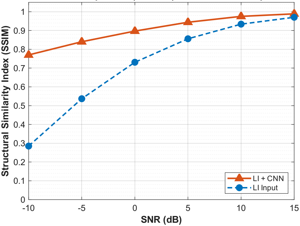
SSIM Comparison (Test Set): LI + CNN vs. LI Input
