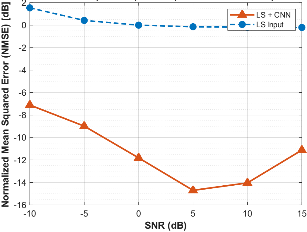
NMSE Comparison (Test Set): LS + CNN vs. LS Input
