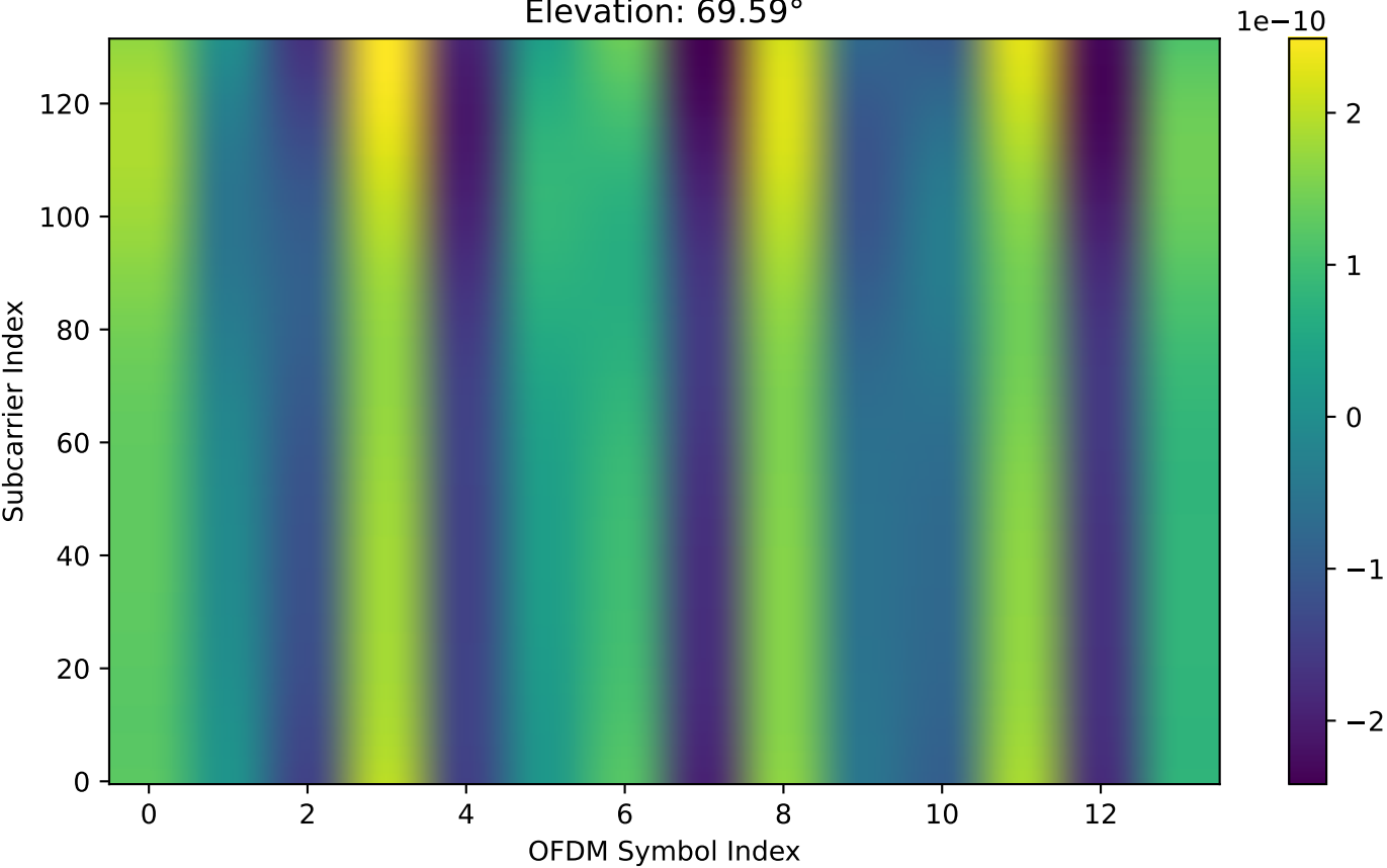
Original Perfect Channel (Full Doppler): Real Part of Channel 0 (DUR) Elevation: 69.59^\circ
