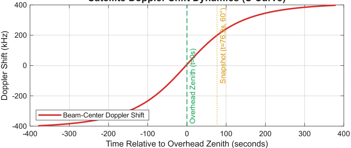
Satellite Doppler Shift Dynamics (S-Curve)
