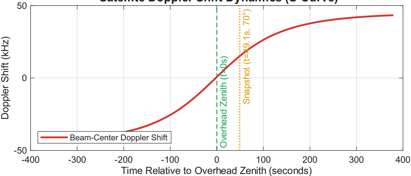
Satellite Doppler Shift Dynamics (S-Curve)
