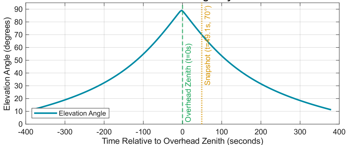
Satellite Elevation Angle Dynamics
