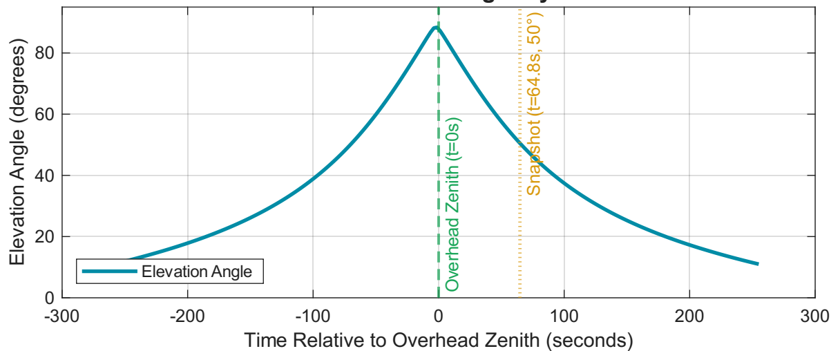
Satellite Elevation Angle Dynamics
