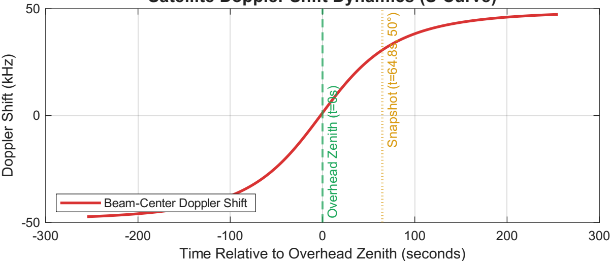
Satellite Doppler Shift Dynamics (S-Curve)
