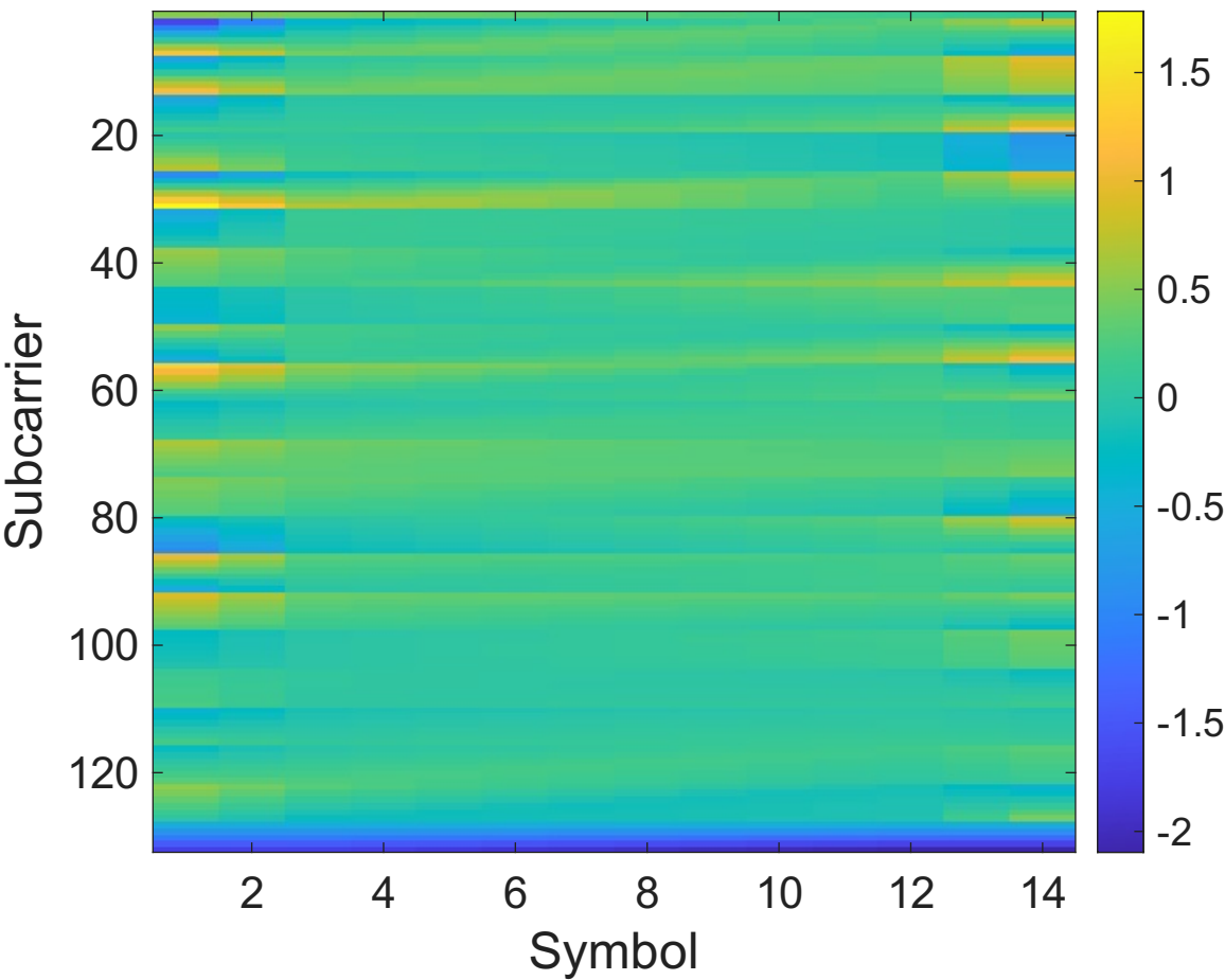
Linear Interpolation Estimated Channel H_{li} (Sample 1) \times 10^{-7}
