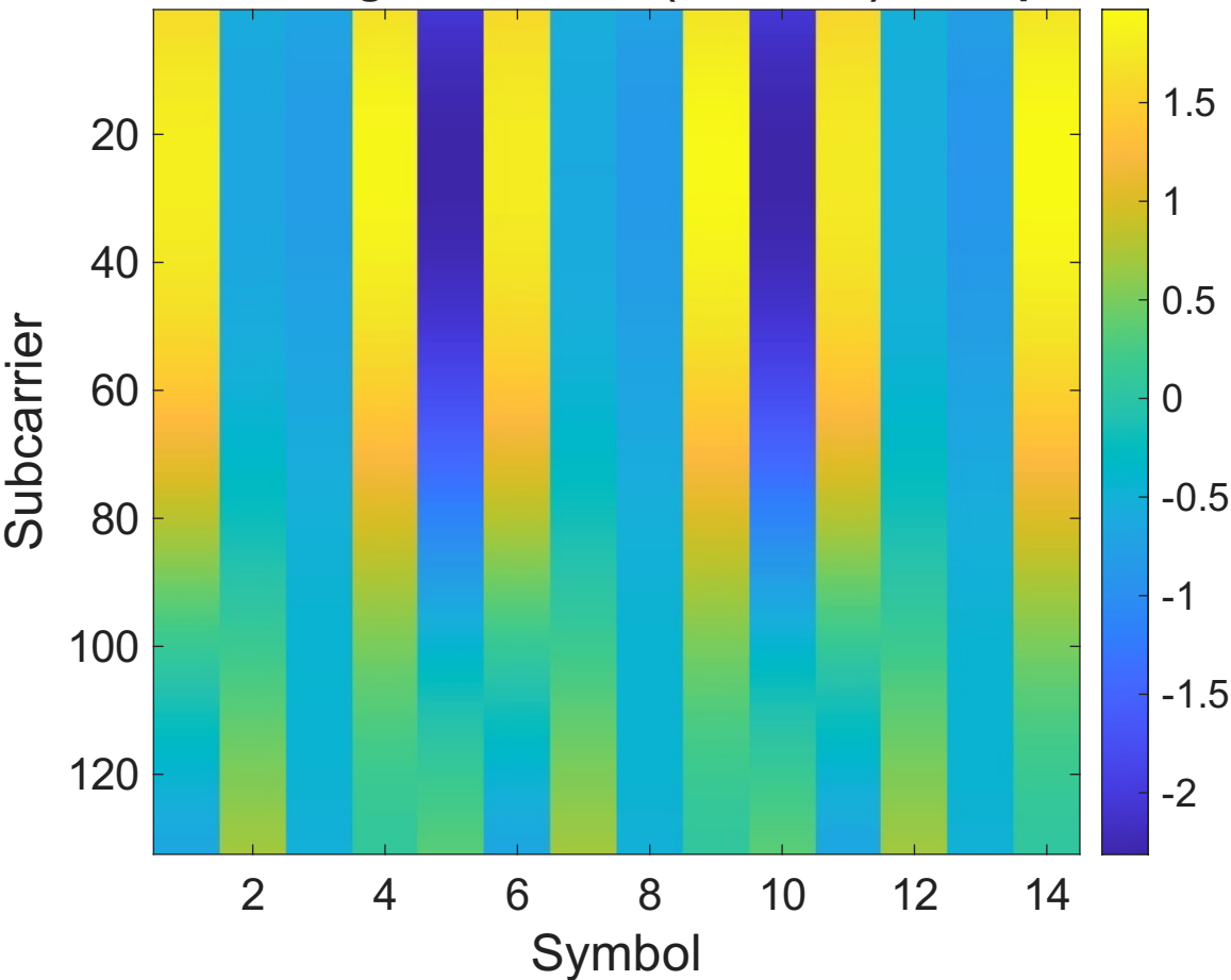
Perfect Original Channel (Real Part) - Sample 1 \times 10^{-8}
