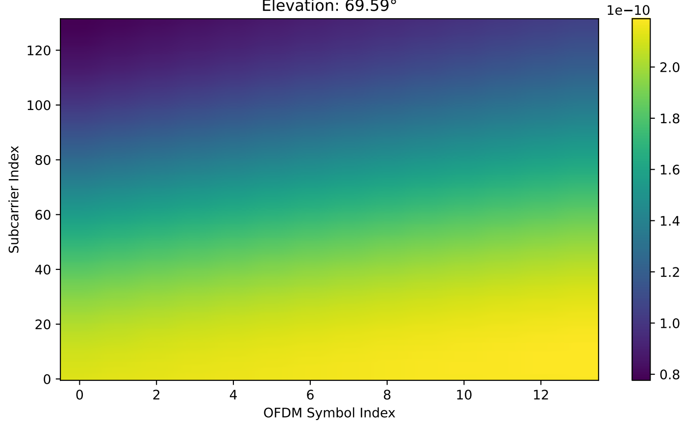
Effective Compensated Channel (Precompensated Satellite Doppler): Real Part of Channel 0 (SUR)
