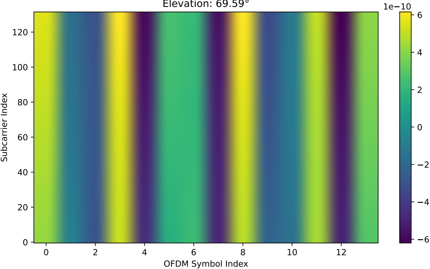
Original Perfect Channel (Full Doppler): Real Part of Channel 0 (SUR) Elevation: 69.59^\circ
