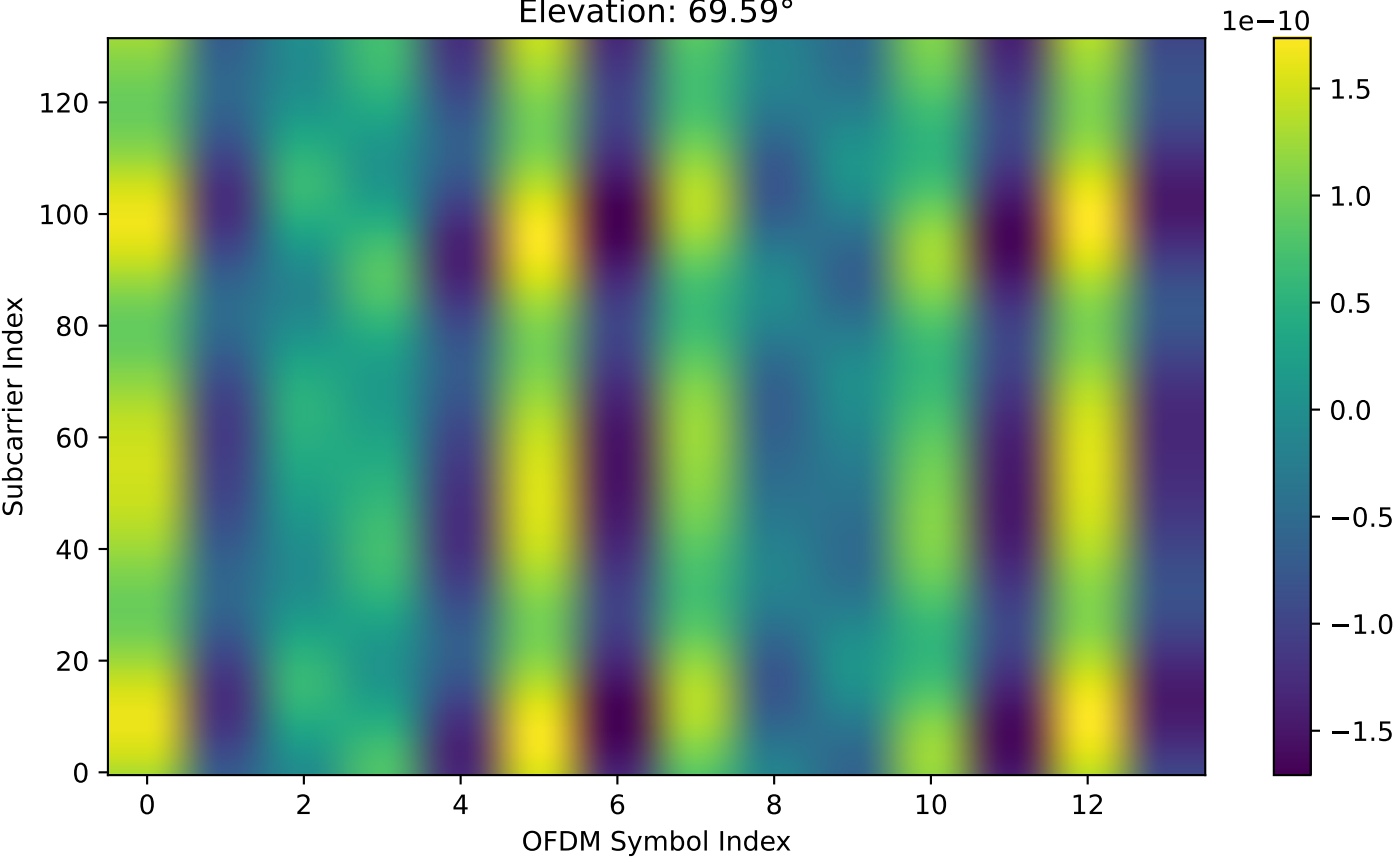
Original Perfect Channel (Full Doppler): Real Part of Channel 0 (URB) Elevation: 69.59^\circ
