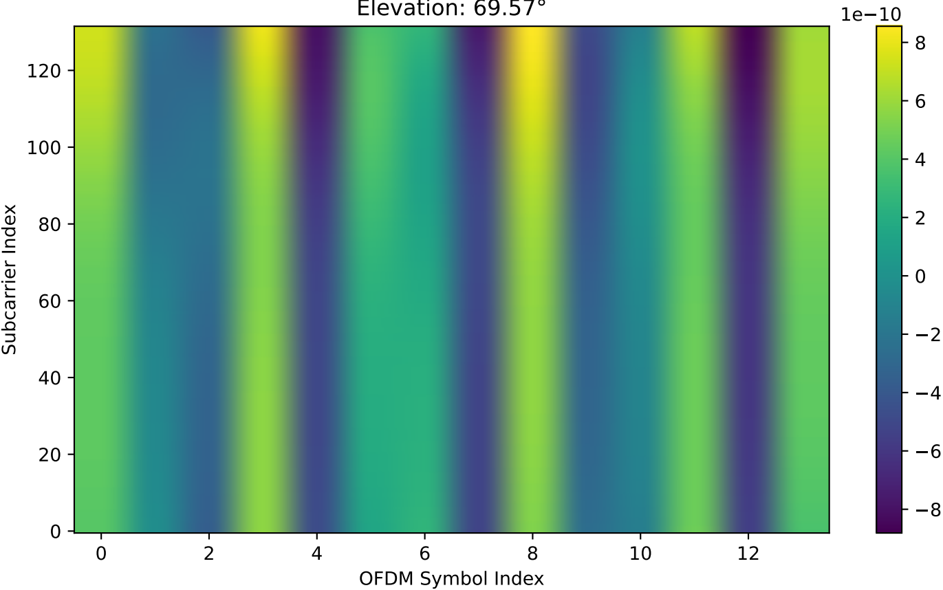
Original Perfect Channel (Full Doppler): Real Part of Channel 0 (DUR) Elevation: 69.57^\circ
