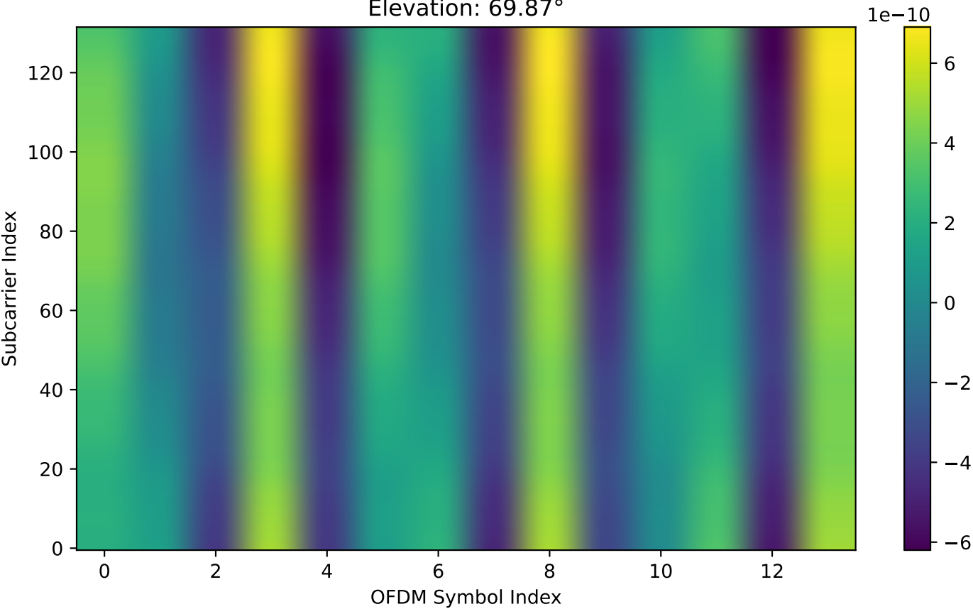
Original Perfect Channel (Full Doppler): Real Part of Channel 1 (DUR) Elevation: 69.87^\circ
