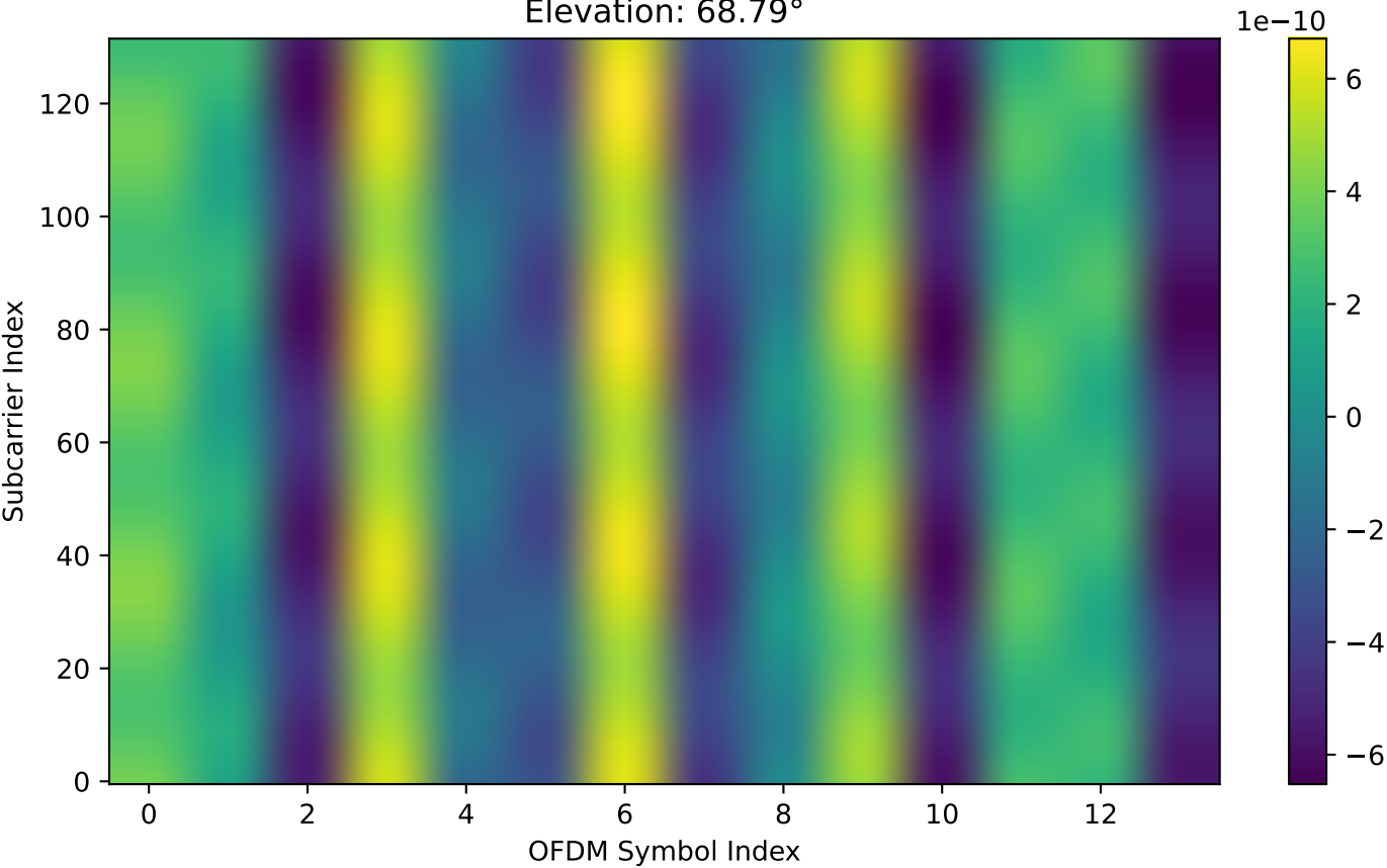
Original Perfect Channel (Full Doppler): Real Part of Channel 2 (DUR) Elevation: 68.79^\circ
