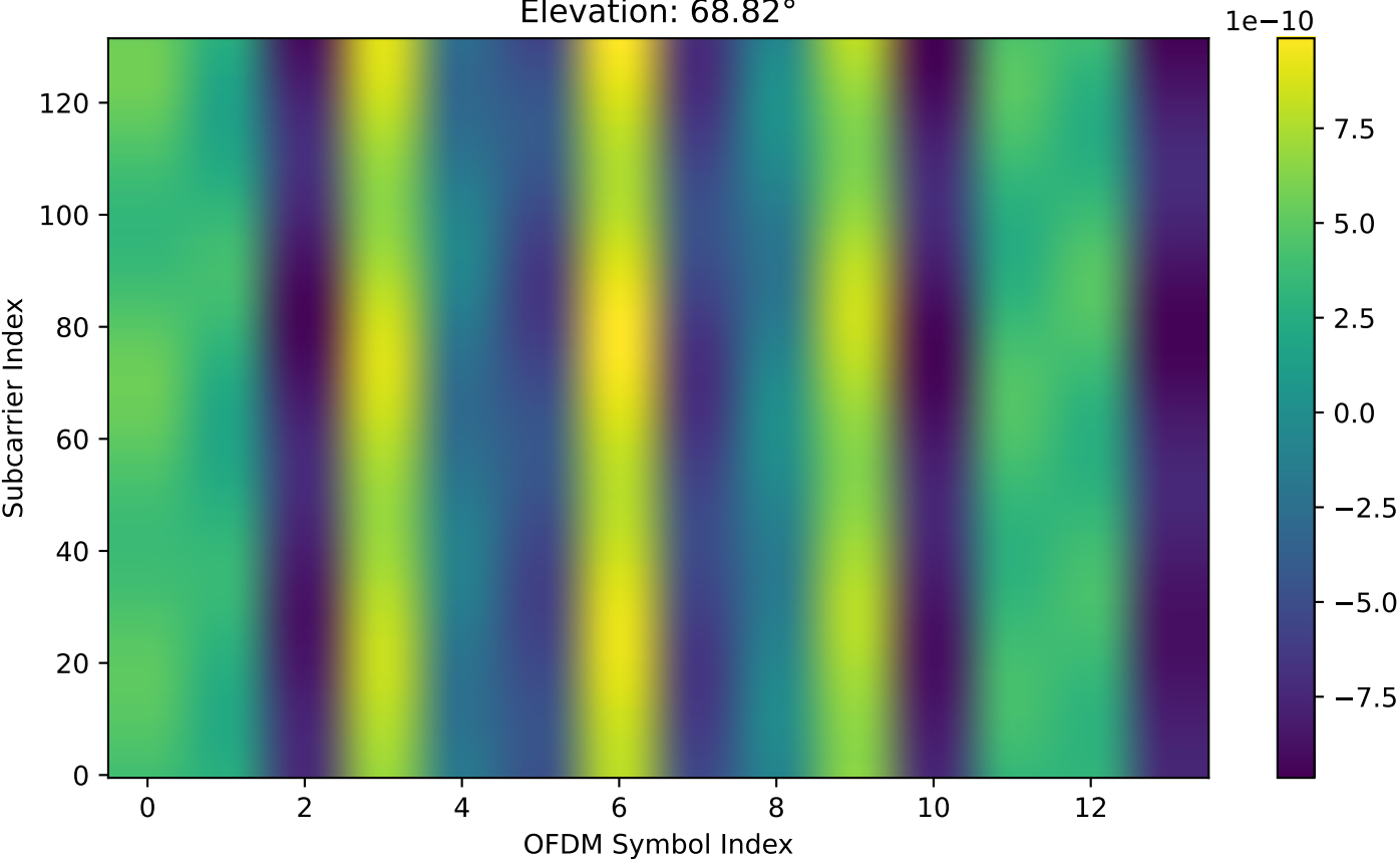
Original Perfect Channel (Full Doppler): Real Part of Channel 3 (DUR) Elevation: 68.82^\circ
