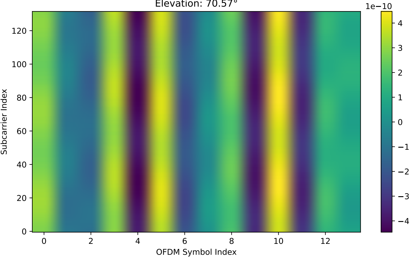
Original Perfect Channel (Full Doppler): Real Part of Channel 4 (DUR) Elevation: 70.57^\circ
