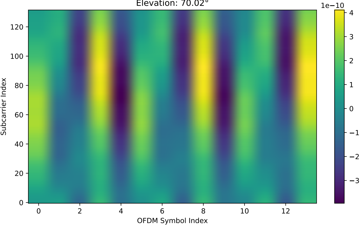
Original Perfect Channel (Full Doppler): Real Part of Channel 5 (DUR) Elevation: 70.02^\circ
