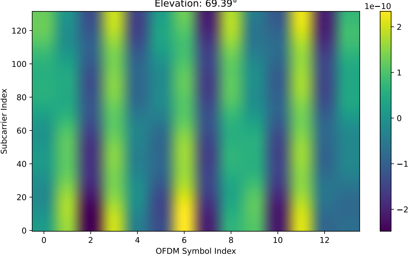
Original Perfect Channel (Full Doppler): Real Part of Channel 7 (DUR) Elevation: 69.39^\circ
