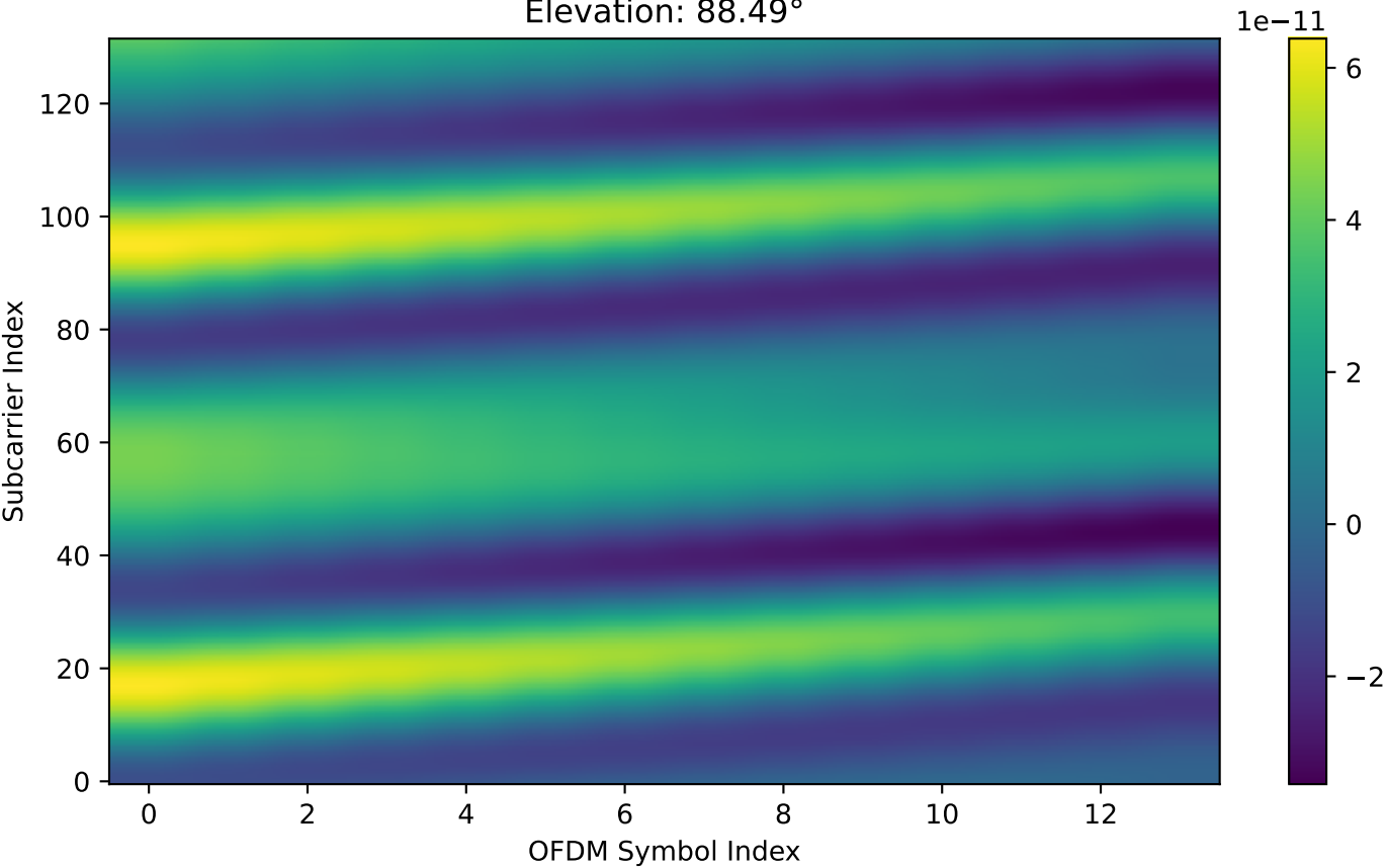
Precompensated Doppler: Real Part of Channel 0 (DUR) Elevation: 88.49°
