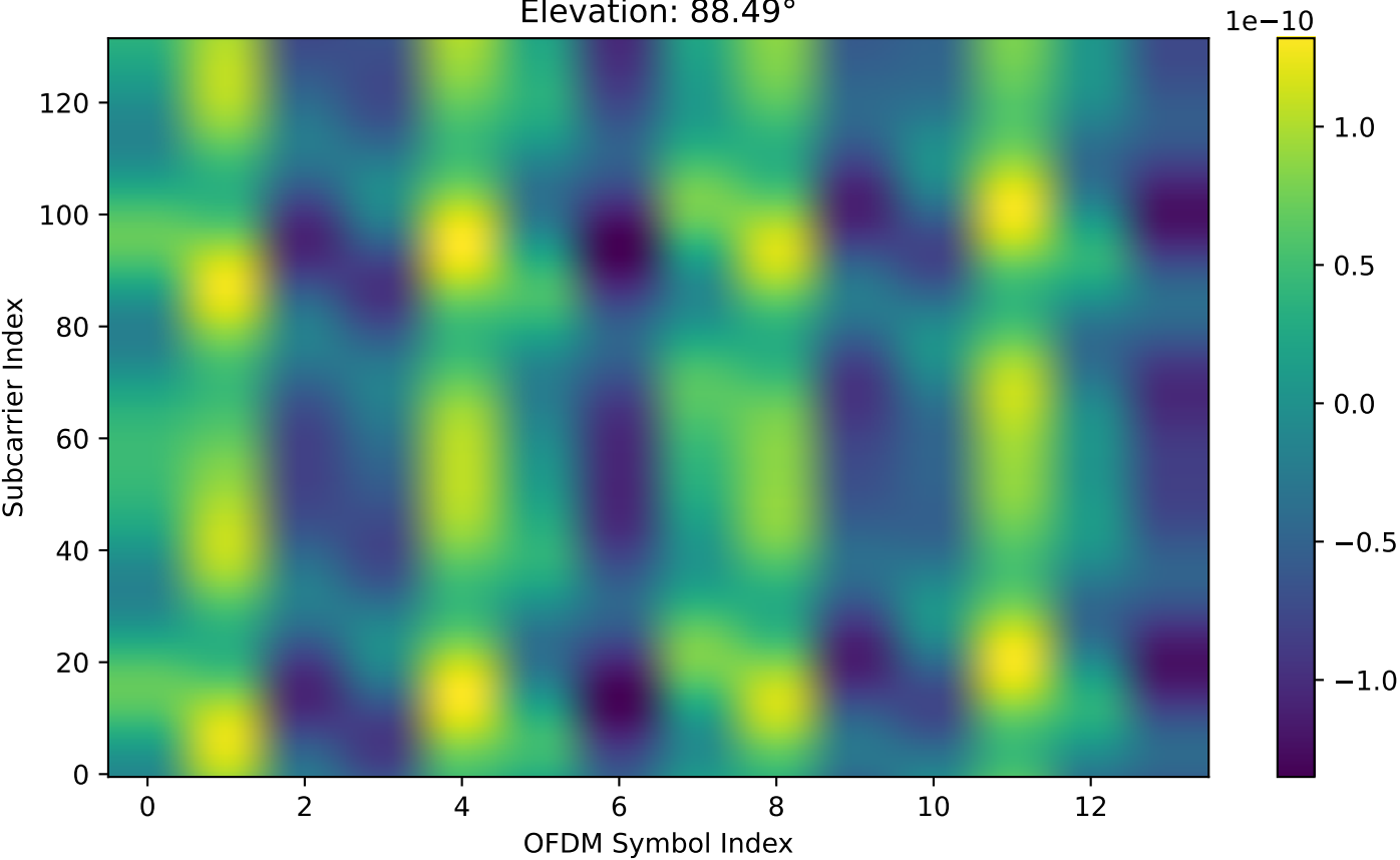
Full Doppler: Real Part of Channel 0 (DUR) Elevation: 88.49°
