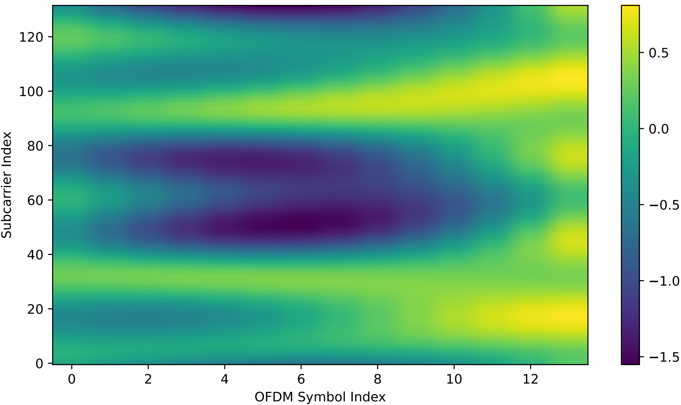
Precompensated Doppler: Real Part of Channel 0 (DUR) Elevation: 88.49°
