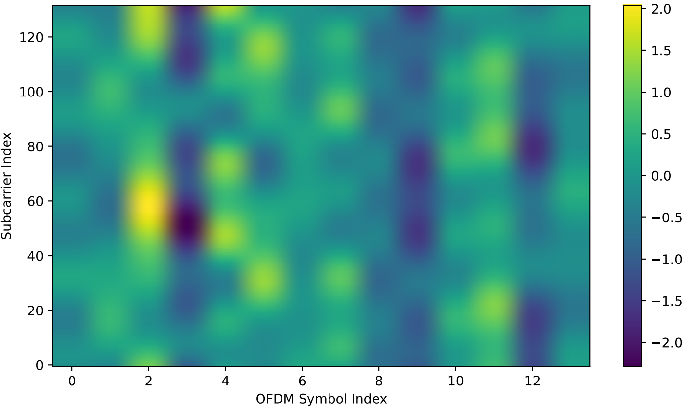
Full Doppler: Real Part of Channel 0 (NTN-TDL-A) Elevation: 88.34°
