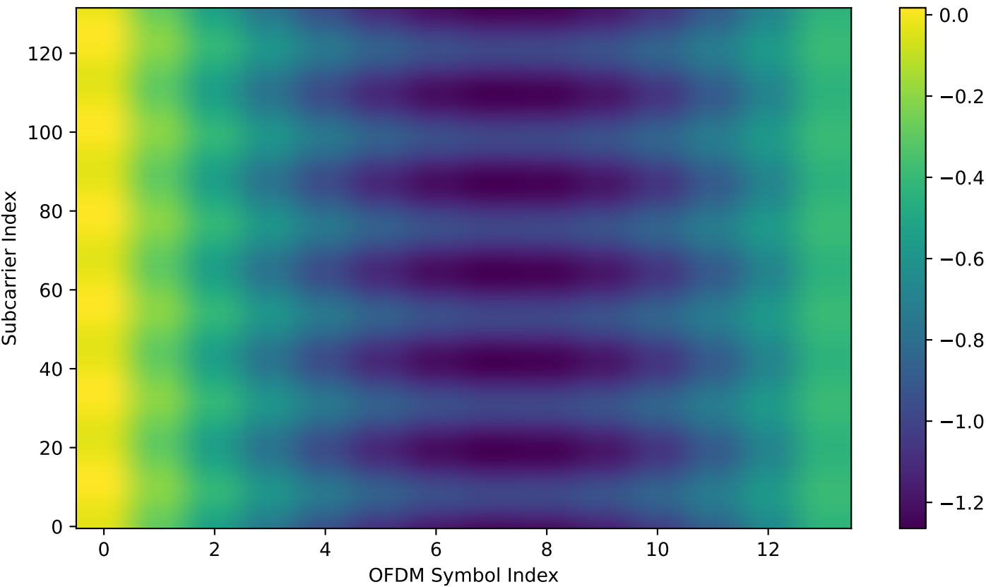
Precompensated Doppler: Real Part of Channel 0 (NTN-TDL-C) Elevation: 88.34°
