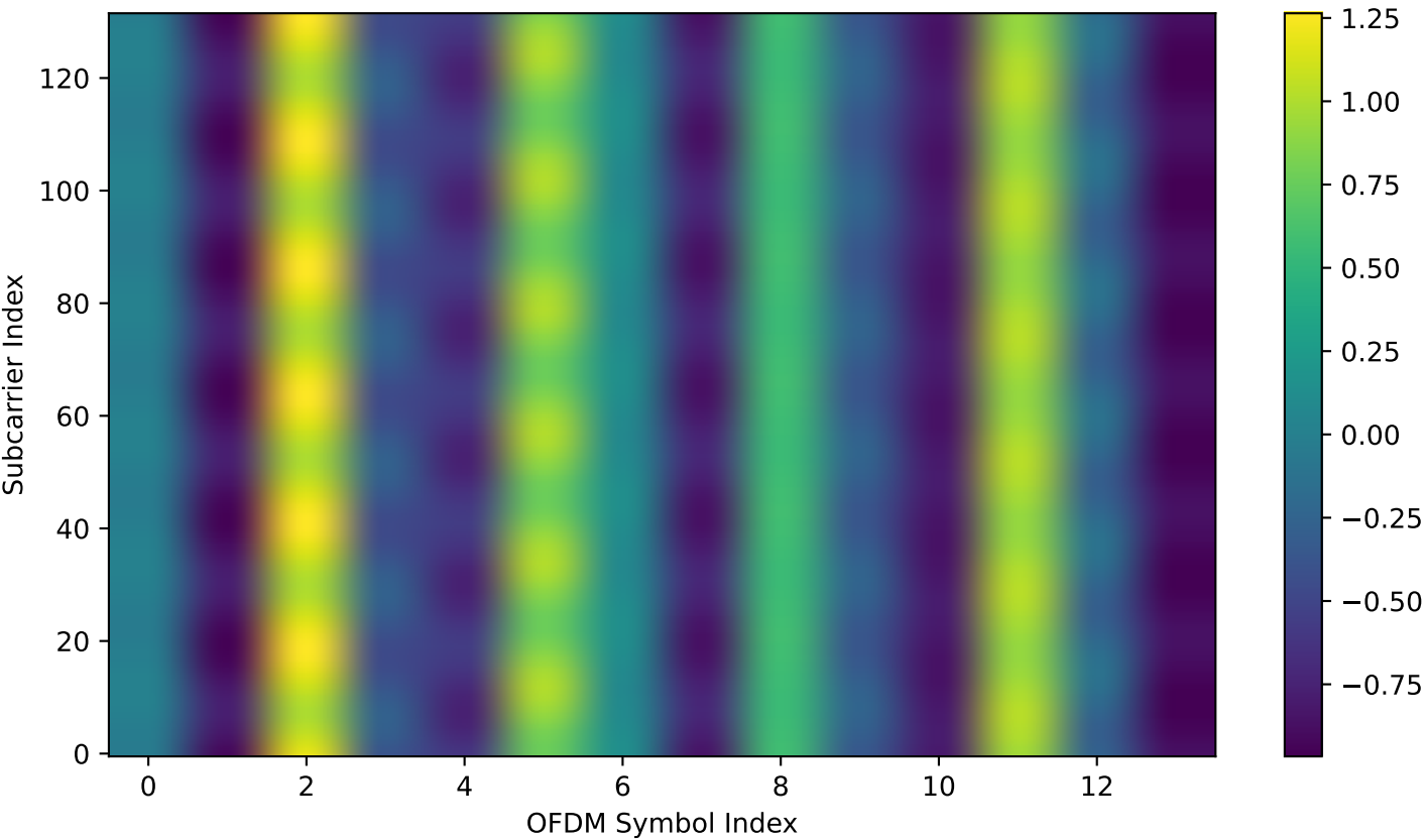
Full Doppler: Real Part of Channel 0 (NTN-TDL-C) Elevation: 88.34°
