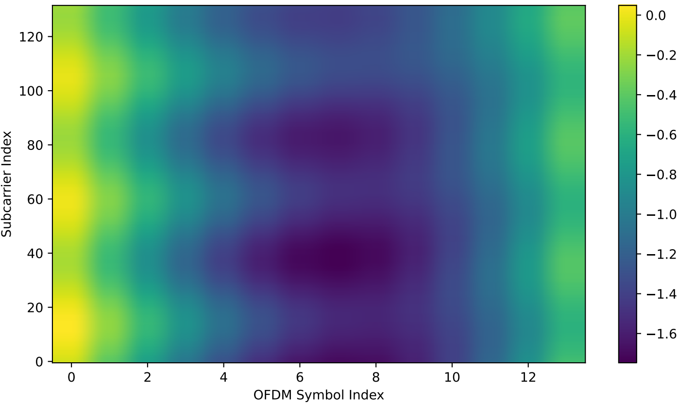
Precompensated Doppler: Real Part of Channel 0 (NTN-TDL-D) Elevation: 88.34°
