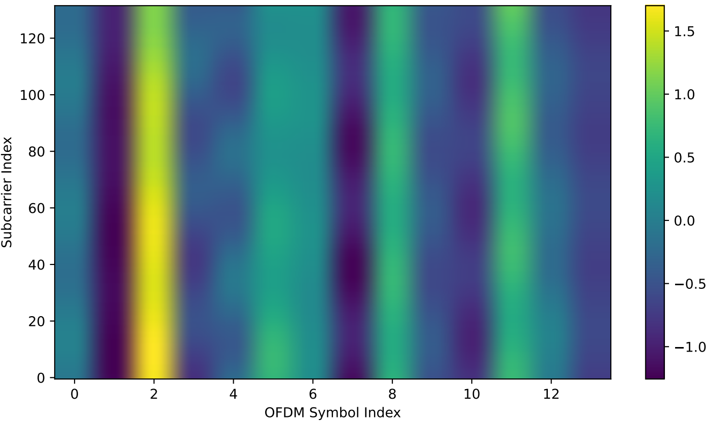
Full Doppler: Real Part of Channel 0 (NTN-TDL-D) Elevation: 88.34°
