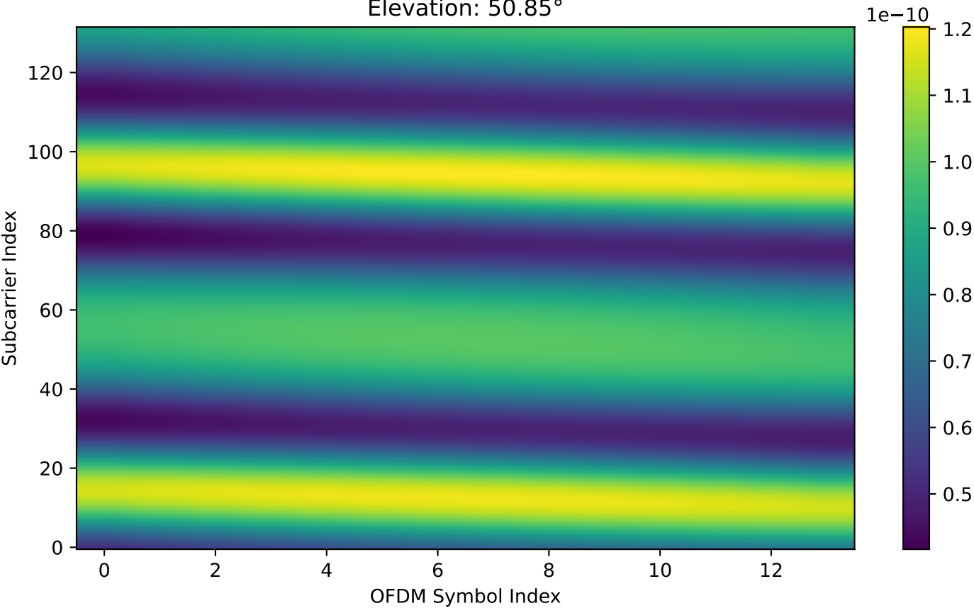
Precompensated Doppler: Real Part of Channel 0 (DUR) Elevation: 50.85°
