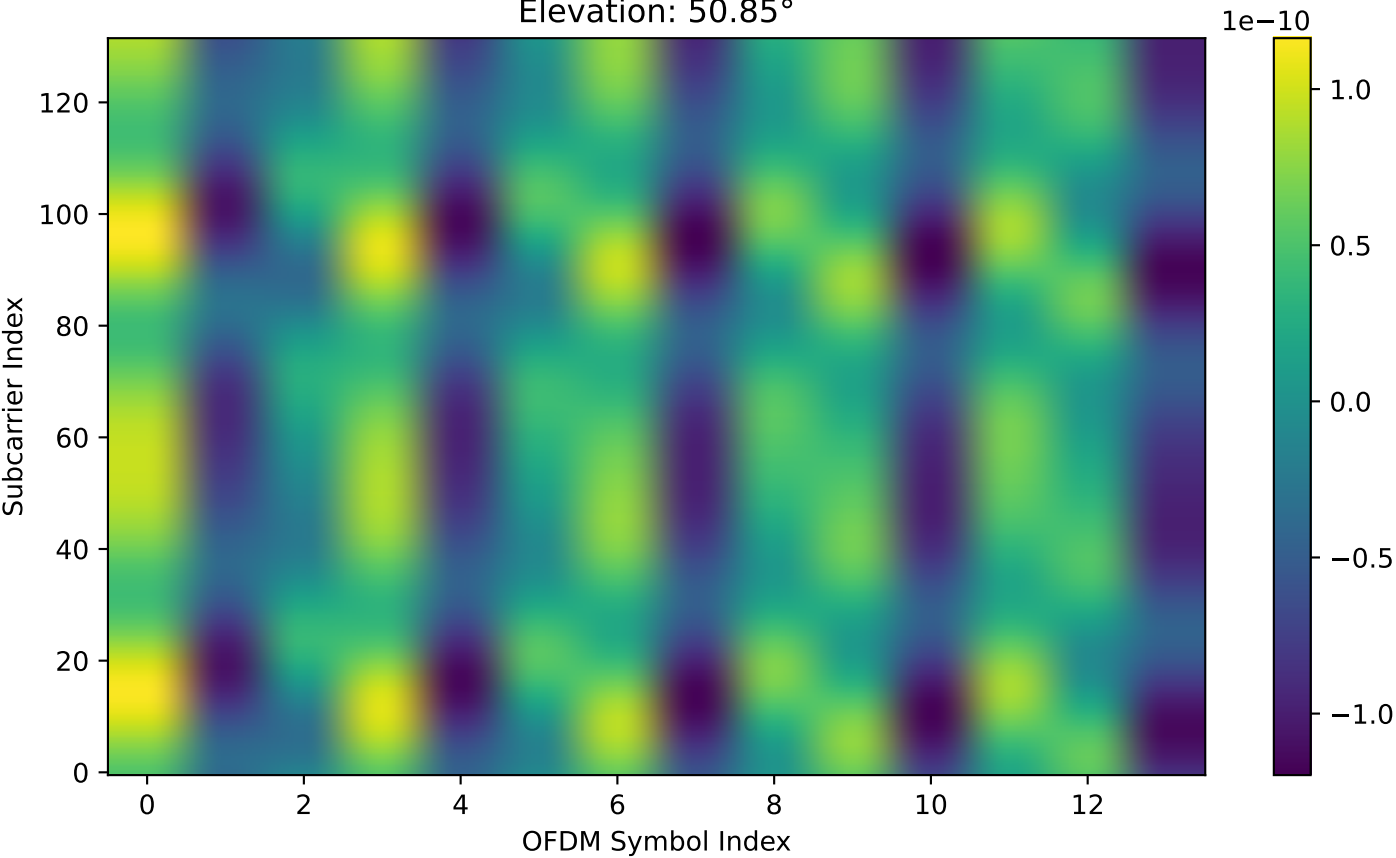
Full Doppler: Real Part of Channel 0 (DUR) Elevation: 50.85°
