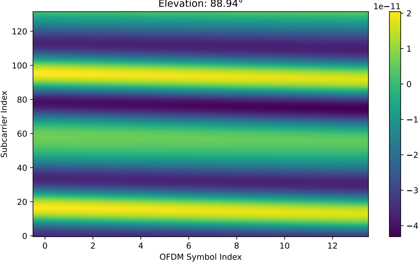
Precompensated Doppler: Real Part of Channel 0 (DUR) Elevation: 88.94°
