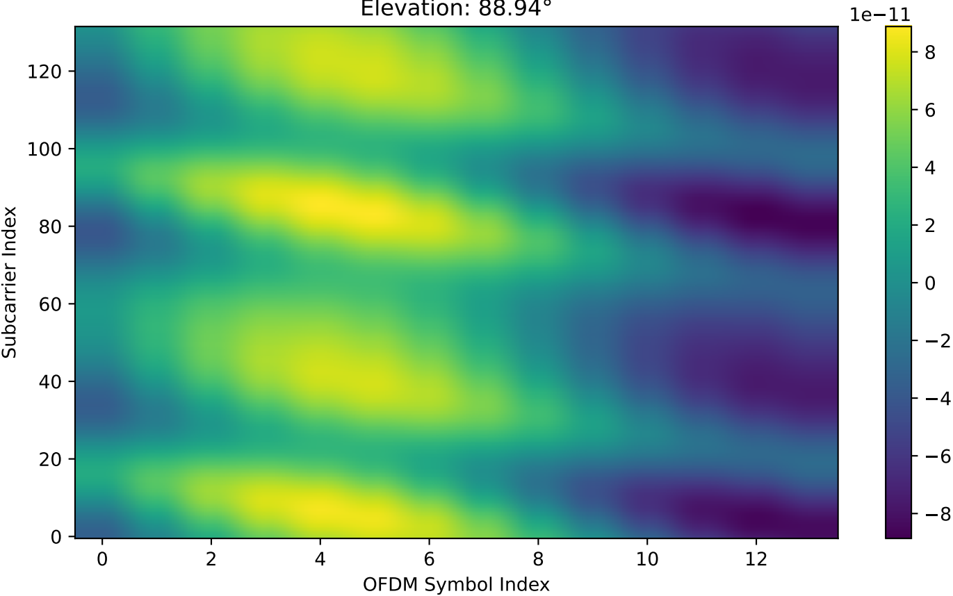
Full Doppler: Real Part of Channel 0 (DUR) Elevation: 88.94°
