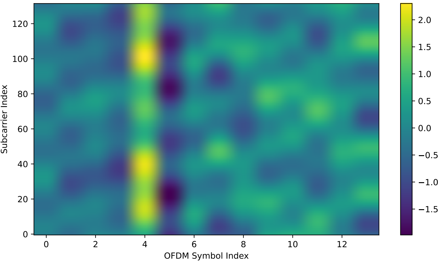
Full Doppler: Real Part of Channel 0 (NTN-TDL-A) Elevation: 50.85°
